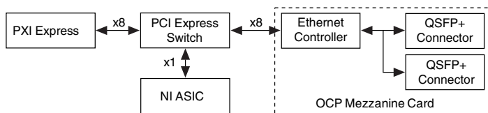
Figure 1. PXIe-8240 Block Diagram
