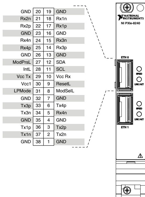
Figure 3. QSFP+ Connector Pinout
