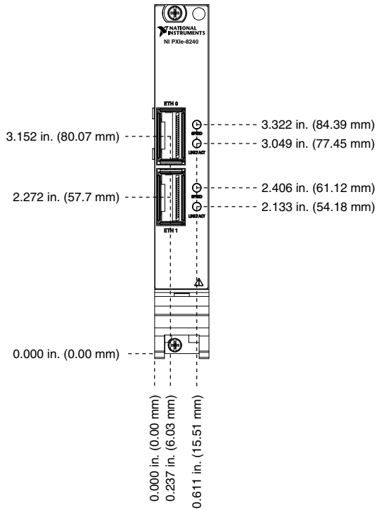
Figure 2. PXIe-8240 Front Panel Layout and Dimensions
